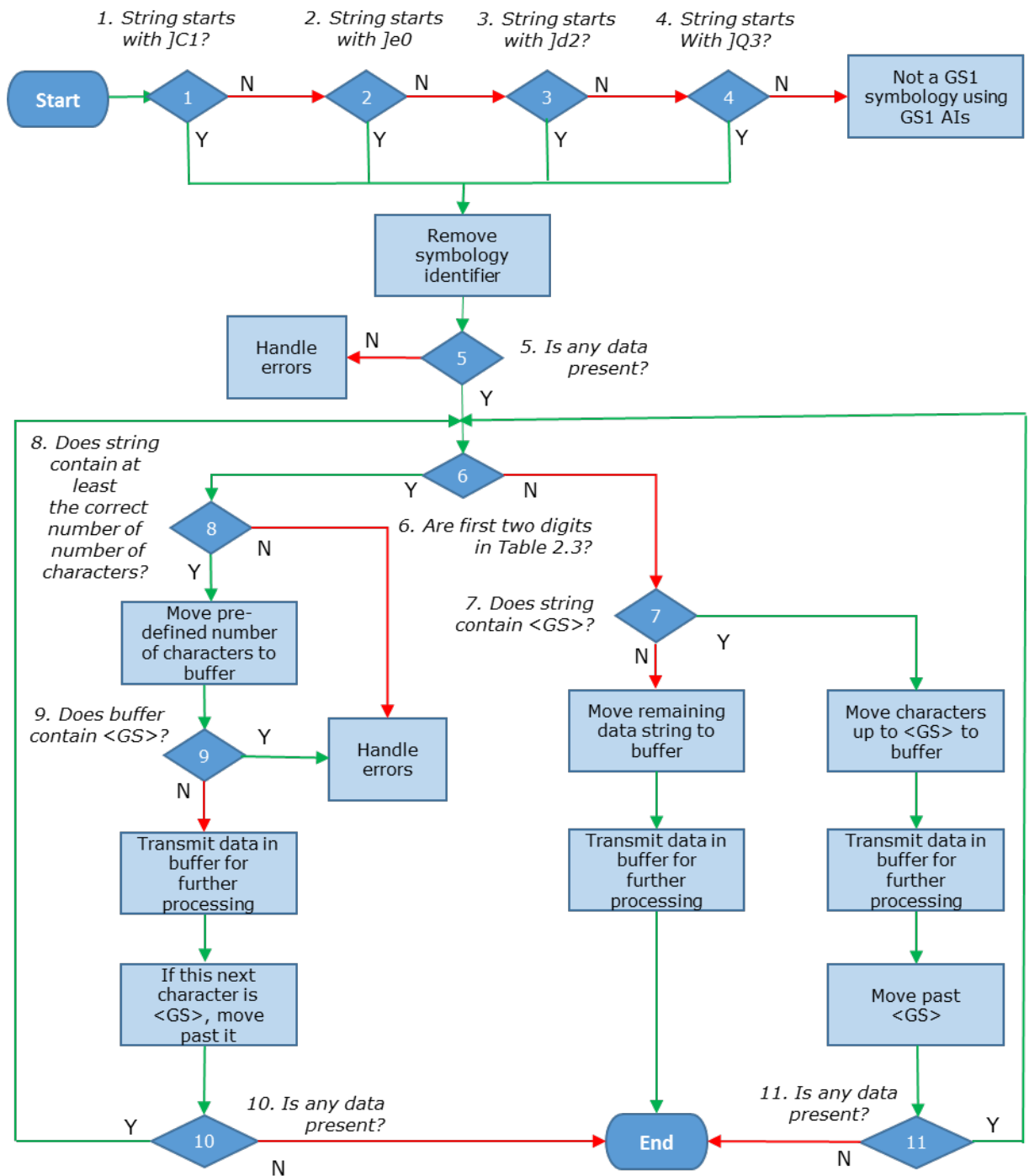
Figure 2-1 Processing of Data from a scanned GS1 DataMatrix symbol
