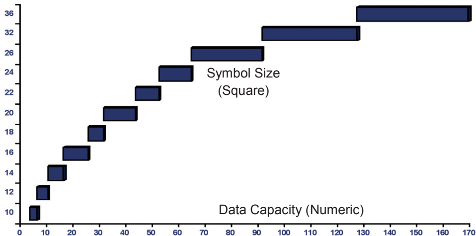
Figure 1-3 Symbol Size vs. Numeric Capacity
